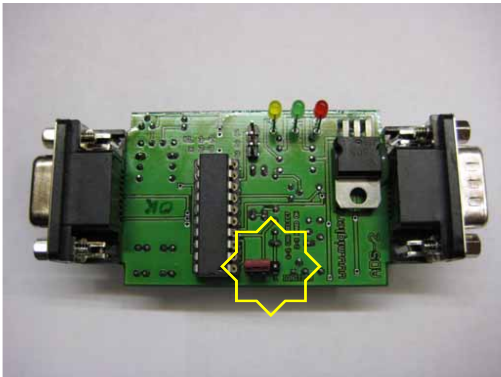
Interface in ADS Mode with ignition (KL15) allways ON
