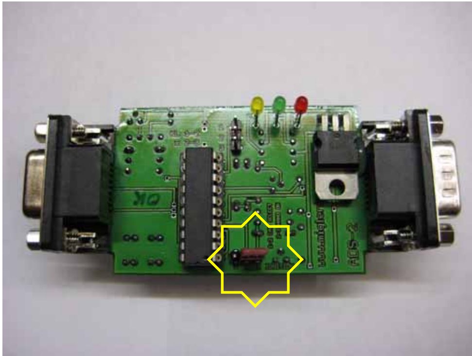
Interface in ADS Mode with ignition (KL15) setting by car
